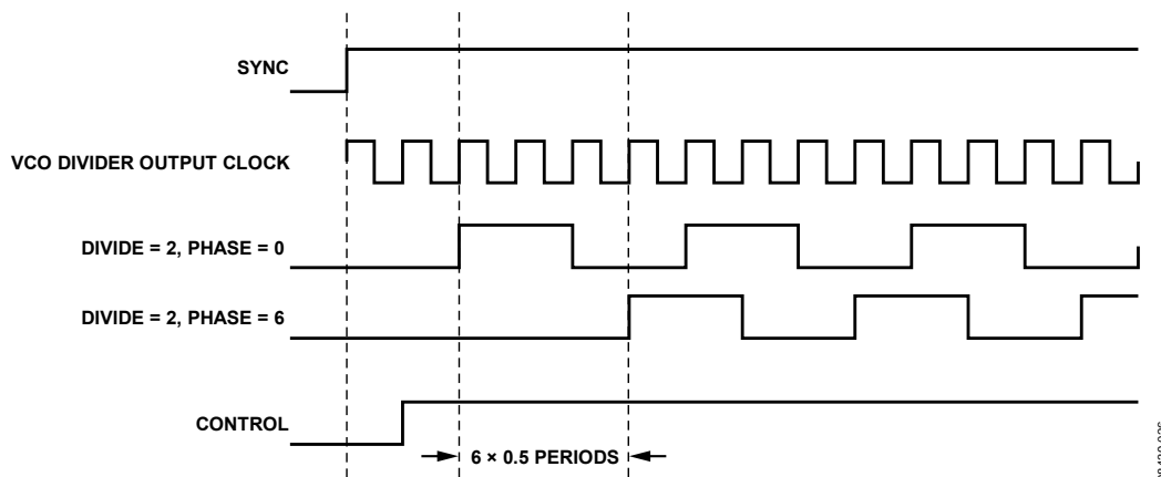
Figure 28. Clock Output Synchronization Timing Diagram
