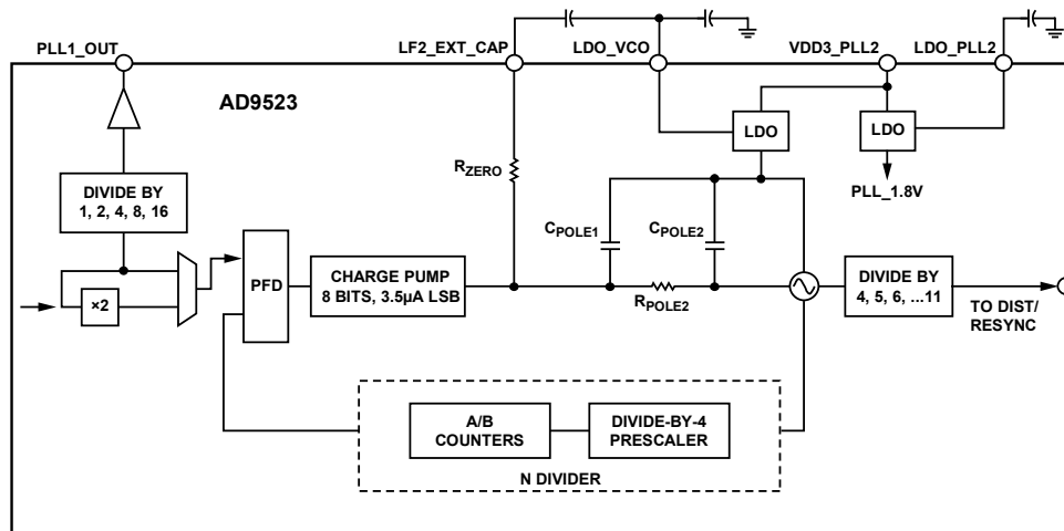
Figure 25. Output PLL (PLL2) Block Diagram
