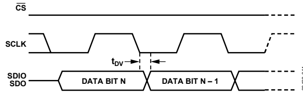
Figure 41. Timing Diagram for Serial Control Port Register Read
