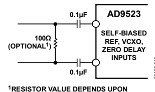
Figure 21. REF, VCXO, and Zero Delay Input Differential Mode
