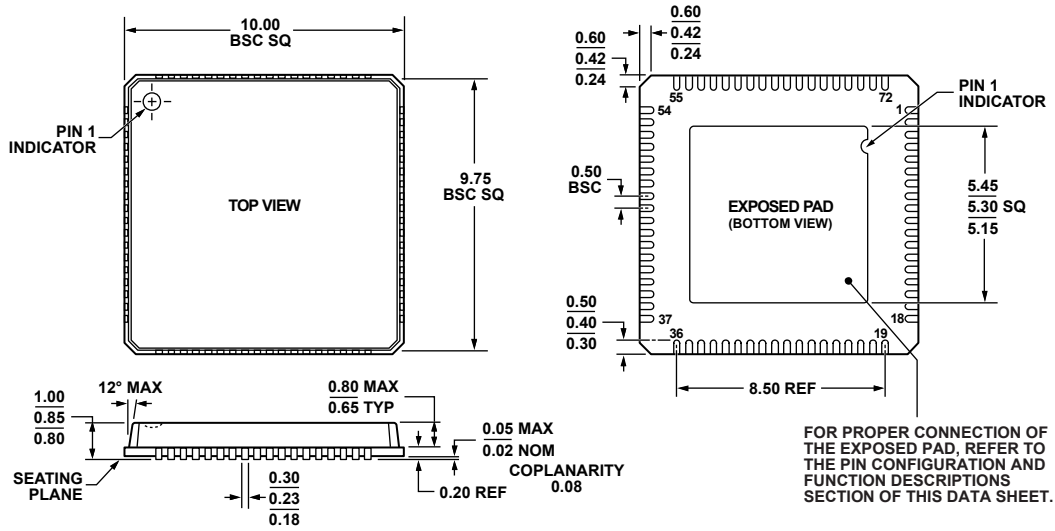
Figure 44. 72-Lead Lead Frame Chip Scale Package [LFCSP_VQ] 10 mm × 10 mm Body, Very Thin Quad (CP-72-6) Dimensions shown in millimeters
