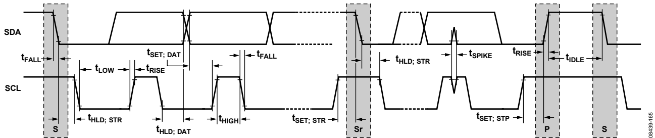
Figure 35. I 2 C Serial Port Timing
