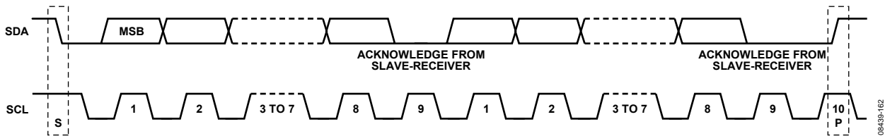
Figure 32. Acknowledge Bit
