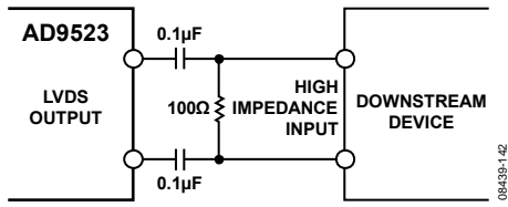
Figure 15. AC-Coupled LVDS Output Driver
