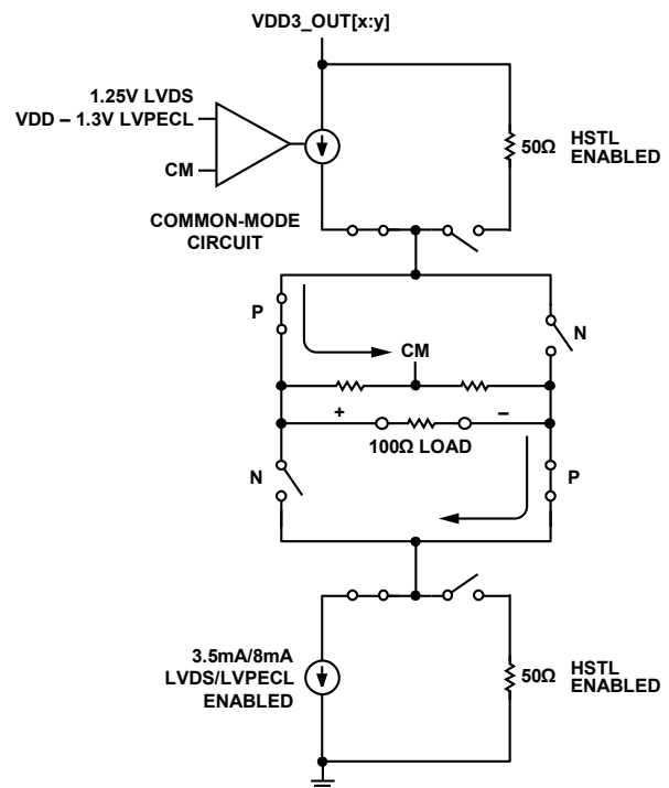
Figure 26. Multimode Driver
