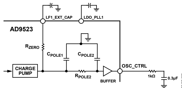
Figure 23. PLL1 Loop Filter
